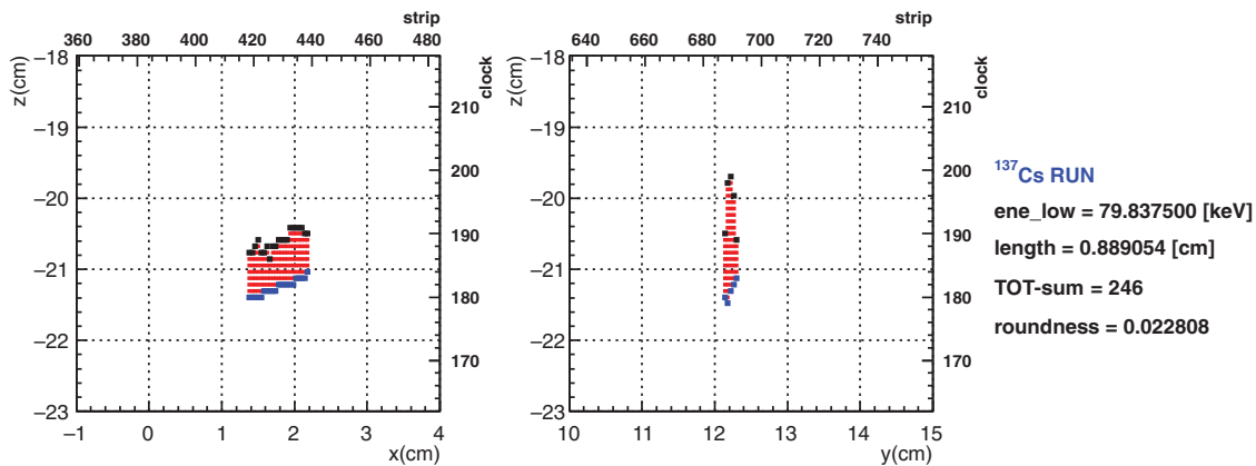
Fig. 6. Track sample of \alpha particle background from \mu -PIC, contaminating a ^{137}\text{Cs} run. This type of event is cut by the roundness cut.
