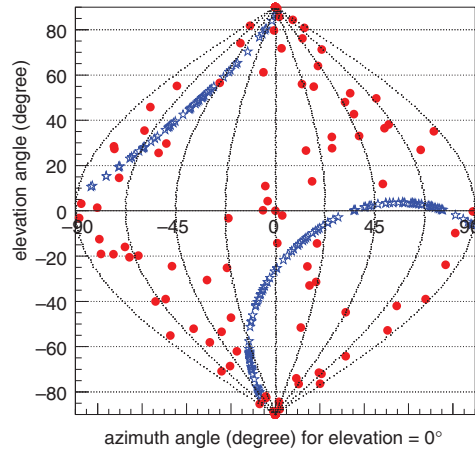
Fig. 14. The directions of nuclear tracks obtained in RUN14 in the 50–400 keV energy range drawn by sinusoidal projection (red). Blue points are the Cygnus direction corresponding to each event. Note that because this analysis does not use head–tail recognition, the range of azimuth angle is up to \pm 90^\circ .
