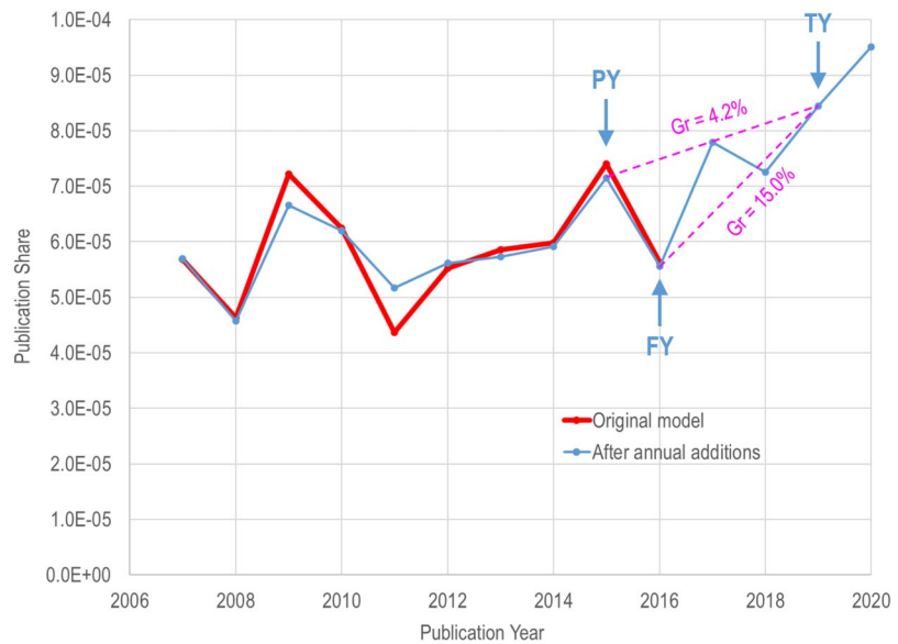
Figure 2. Detailed publication history of RC #5528. Publication share is the fraction of the number of papers from the overall model that are in the cluster in a particular year. Use of publication share normalizes for growth in the database. Two different retrospective actual growth rates as of the target year (TY) 2019 are shown. One is based on the forecast year (FY) 2016 and the other is based on the peak year (PY) 2015.
