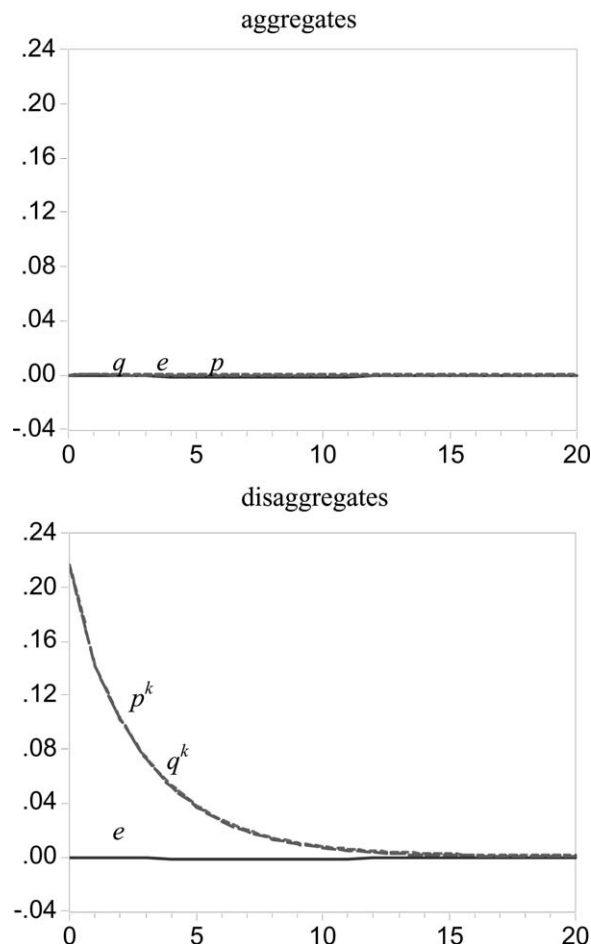
FIGURE 3.—IMPULSE RESPONSE TO q^h SHOCK
