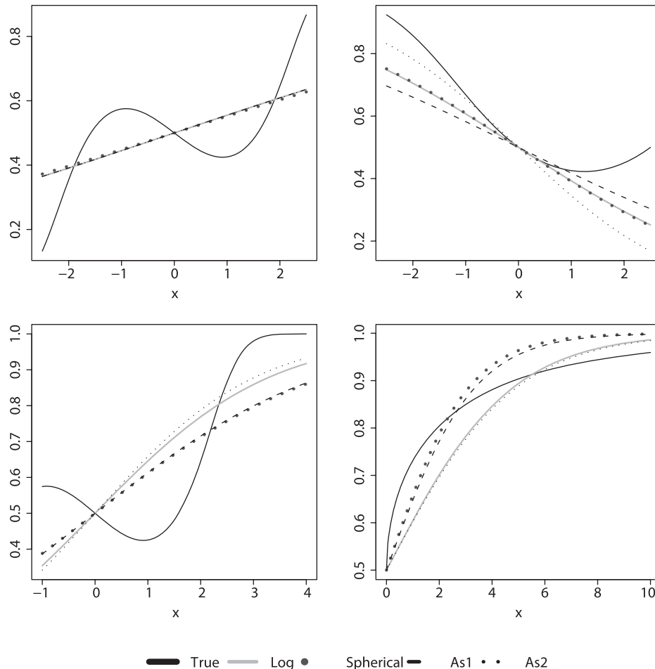
FIGURE 2.—ASYMPTOTIC PROBLEM UNDER MISSPECIFICATION FOR DGPs #1 (UPPER LEFT), #2 (UPPER RIGHT), #3 (LOWER LEFT), AND #4 (LOWER RIGHT)
