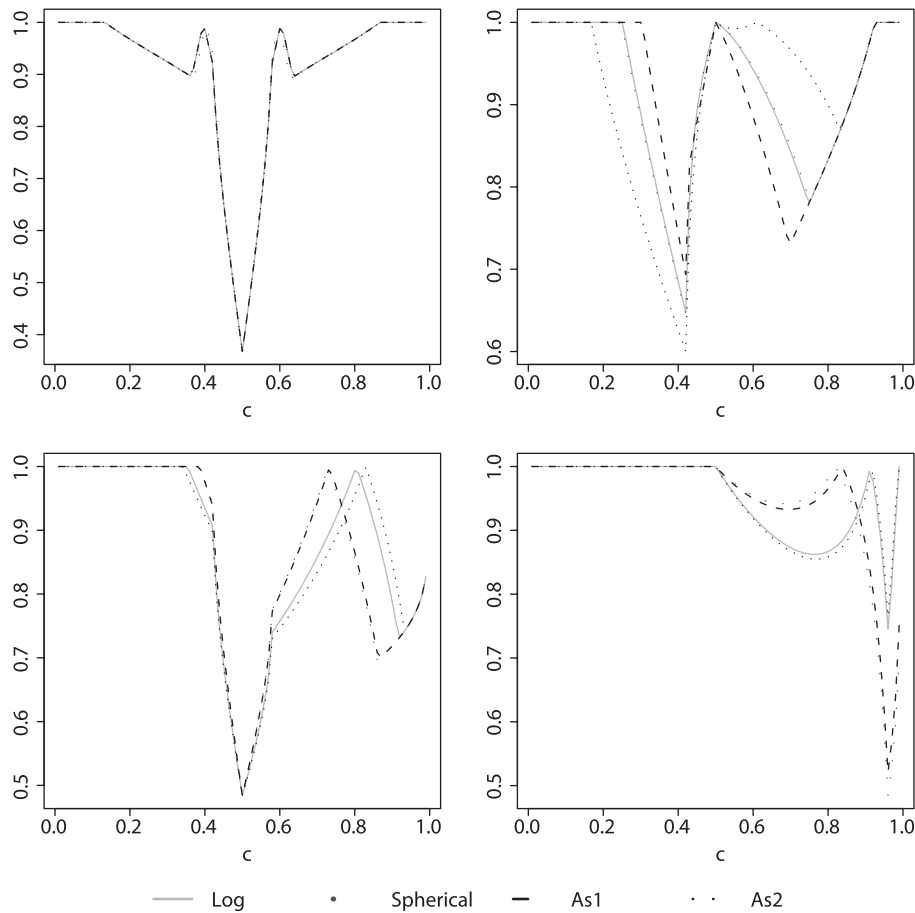
FIGURE 5.—ASYMPTOTIC PROBLEM UNDER MISSPECIFICATION FOR DGPs #1 (UPPER LEFT), #2 (UPPER RIGHT), #3 (LOWER LEFT), AND #4 (LOWER RIGHT)
