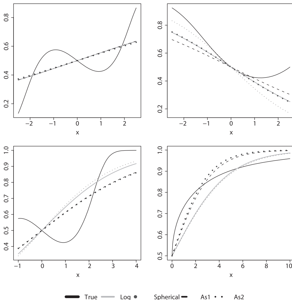
FIGURE 2.—ASYMPTOTIC PROBLEM UNDER MISSPECIFICATION FOR DGPs #1 (UPPER LEFT), #2 (UPPER RIGHT), #3 (LOWER LEFT), AND #4 (LOWER RIGHT)
