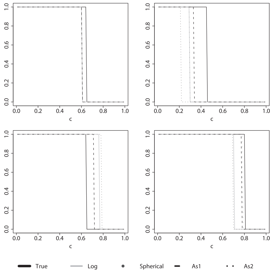
FIGURE 3.—ASYMPTOTIC PROBLEM UNDER MISSPECIFICATION FOR DGPs #1 (UPPER LEFT), #2 (UPPER RIGHT), #3 (LOWER LEFT), AND #4 (LOWER RIGHT)
