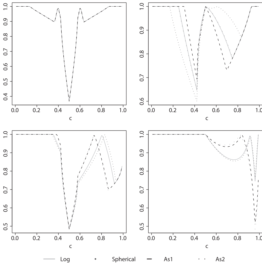
The plots show the probability of correct classification (see equation [12]) for various thresholds c . \theta^* is computed using a sample of size 1,000,000.
