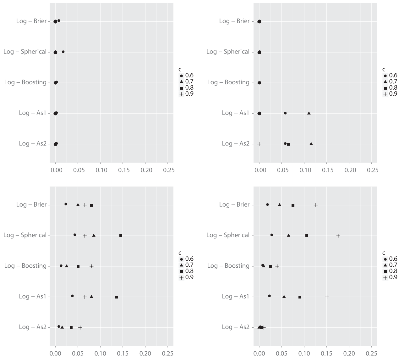
FIGURE 4.—ASYMPTOTIC PROBLEM UNDER MISSPECIFICATION FOR DGPs #1 (UPPER LEFT), #2 (UPPER RIGHT), #3 (LOWER LEFT), AND #4 (LOWER RIGHT)
