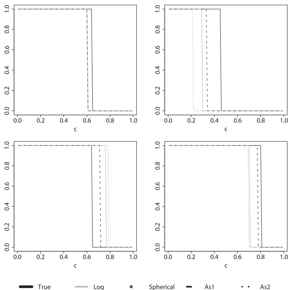
The plots show the classification curves of the conditional probability given x = 2 ( \theta_j^* is computed using a sample of size 1,000,000).
