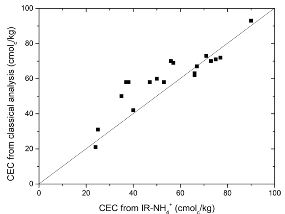
Fig. 7 Example of the relationship between the CEC calculated from \text{NH}_4^+ methods and the CEC measured by the classical method. The samples are from soil series and from various kaolinite-smectite mechanical mixtures. Data adapted and modified from Petit et al. (1998)
