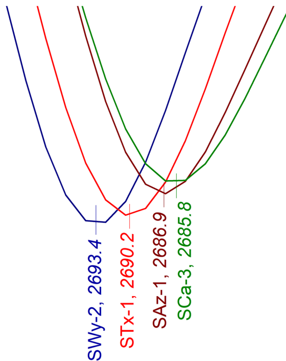
Fig. 14 Position of the \nu\text{O-D}_w 2 nd derivative minima of SWy-2, STx-1, SAz-1, and SCa-3 montmorillonites in their as-received cation forms (cf. Figure 13)
