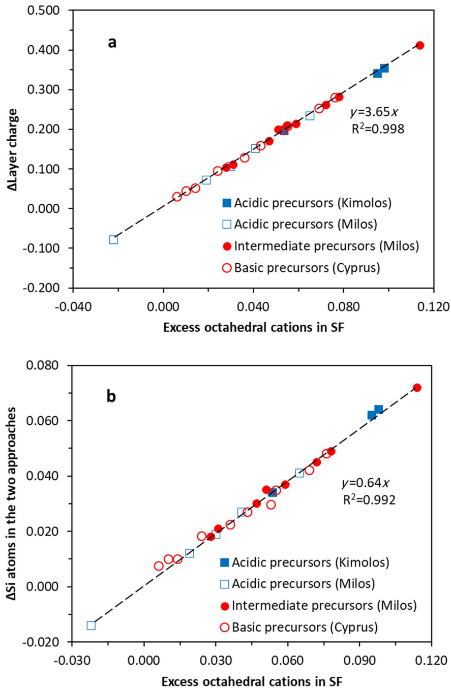
Fig. 1 Excess octahedral cations (e/huc) calculated with the fixed anionic charge approach vs a difference in layer charge calculated by the two approaches and b the difference in Si atoms calculated by the two approaches
