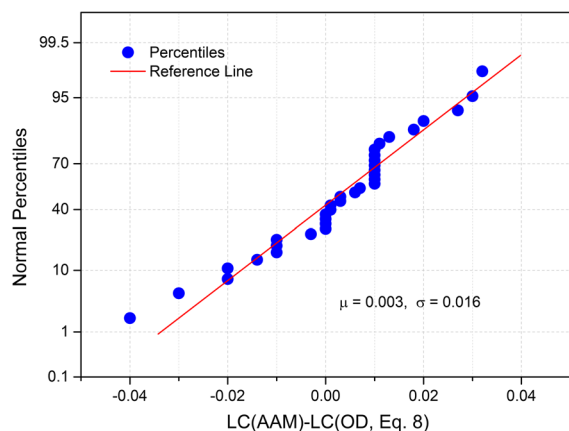
Fig. 15 Validation of the \nu\text{O}-D_w AAM predictions against the independent reference values of bentonite samples from the Kaufhold collection. The normal probability plot of the residuals indicates \sigma=0.016 and \mu=0.003 e/huc, in excellent agreement with the original calibration (Kuligiewicz et al., 2015b)
