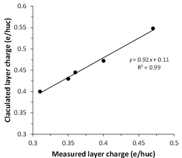
Fig. 11 Correction of the layer charge for smectites with a predominantly tetrahedral charge
