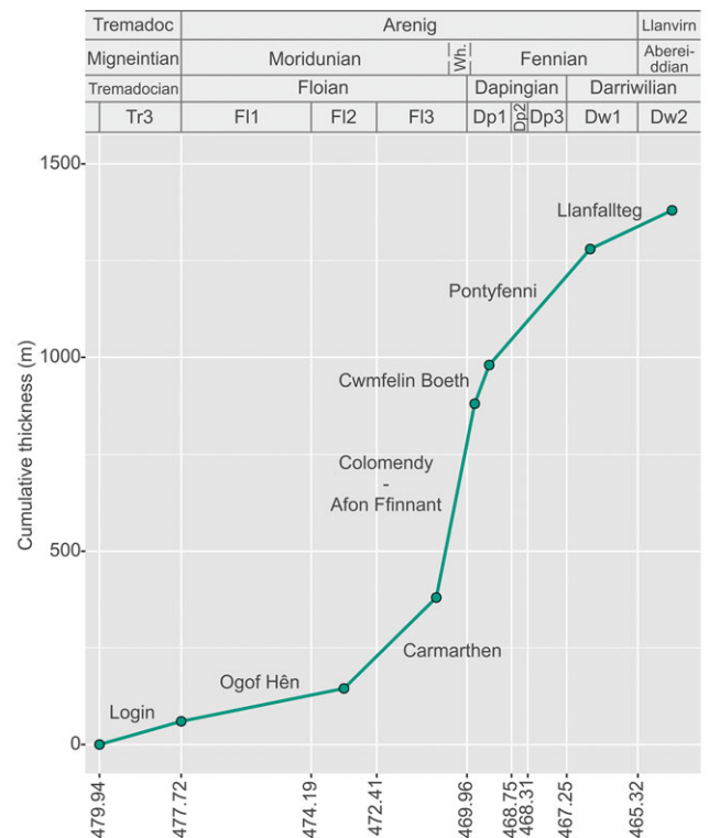
Fig. 11. (Colour online) Cumulative thickness curve for the upper Tremadocian to middle Darriwilian succession in South Wales based on thicknesses in Table 1.
