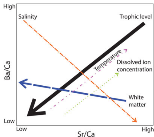
FIGURE 6. Summary of factors affecting Sr/Ca and Ba/Ca ratios compiled from the literature discussed in this study. The arrow direction indicates an increase in the corresponding variable, while the weight represents the relative importance of that variable in our interpretations. The most important variables are trophic level followed by white matter composition, with salinity followed by dissolved ion concentration (Bath et al. 2000; Kraus and Secor 2003) and temperature providing a limited influence on our results.
