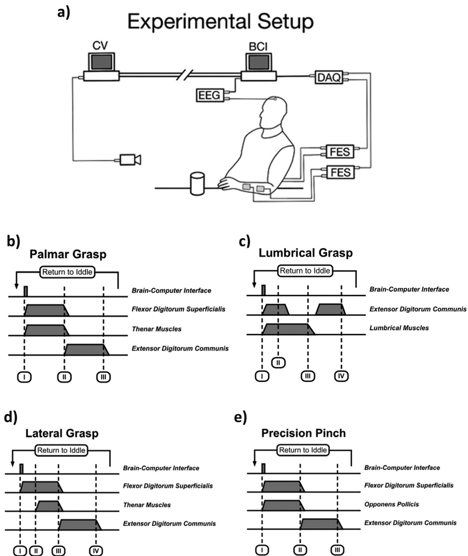
Figure 1. Experimental setup. The computer vision (CV) system and brain-computer interface (BCI) were implemented as two independent systems that could communicate with each other through TCP/IP (transmission control protocol/Internet protocol) networking protocols. The CV system first identified objects placed on a table in front of the participant, determined the grasp necessary to manipulate it, then provided the required grasp to the BCI system. The BCI configured the functional electrical stimulation (FES) system to produce the intended movement. The FES system was implemented using two four-channel electrical stimulators (each capable of producing two different grasps). The BCI used a single EEG electrode. Triggering of the stimulation sequences started when the BCI was activated (event I in figures b, c, d, and e). Activation and deactivation of the stimulation was done gradually by ramping up (or down) its intensity. The facilitated movements included palmar grasp (b), lumbrical grasp (c), lateral grasp (d), and precision pinch (e). All stimulation sequences lasted 8 seconds and ended by facilitating hand opening. This position (opened hand) was sustained for 3 seconds after which the system would return automatically to an idle state, waiting for the next BCI activation.
