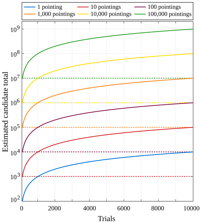
Figure 3. Candidate numbers predicted by equation (4) (using n_\sigma = 7 and n_\sigma^{\max} = 100 ), varied according to the total number of survey pointings for a single beam receiver. Coloured dashed lines indicate the total number of candidates returned when using a conservative C = 100 cut. The corresponding solid colour lines indicate the total number of candidates returned when the cut is discarded. The solid lines are truncated such that they begin where C = 100 to avoid overlapping lines complicating the plot.
