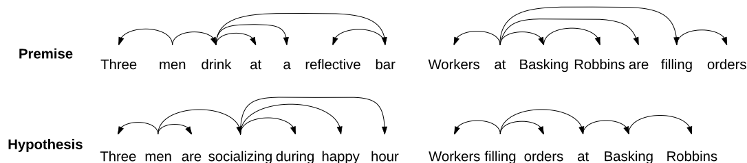
Figure 5: Dependency trees induced by our model on the SNLI test set.
