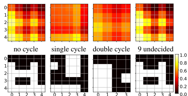
Figure 4: Mean GPLL (top row) and SVM (bottom row) predictions over 25 repeats. Probability that the argument on the horizontal axis \succ the argument on the vertical axis.
