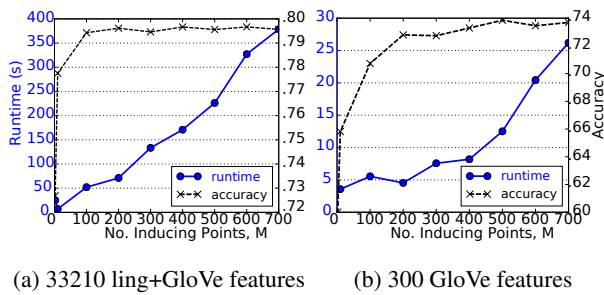
Figure 6: Effect of varying M on accuracy and runtime (training+prediction) of GPLL for UKPCConvArgStrict. Means over 32 runs.
