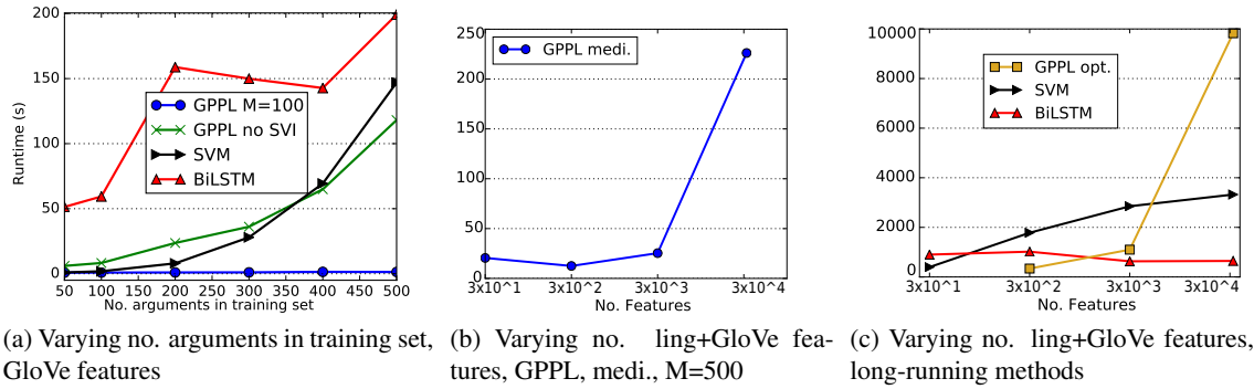
Figure 5: Runtimes for training+prediction on UKPCConvArgStrict with different subsamples of data. Means over 32 runs. Note logarithmic x-axis for (b) and (c).
