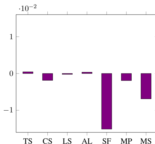
Figure 8: Correlation coefficients between segmentation accuracy and the typological factors in the linear regression model. The factors are training set size (TS), character set size (CS), lexicon size (LS), average word length (AL), segmentation frequency (SF), multitoken word portion (MP) and multitoken word size (MS).
