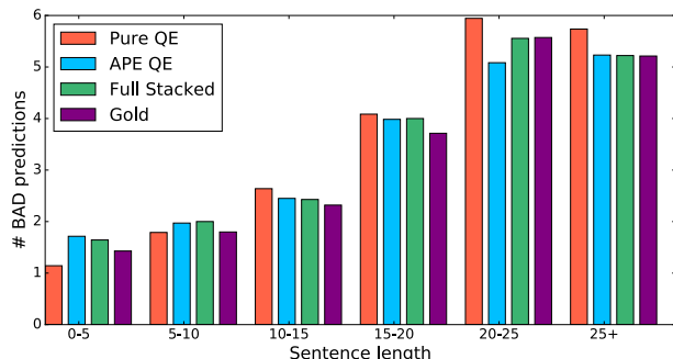
Figure 3: Averaged number of words predicted as BAD by the different systems in the WMT16 gold dev set, for different bins of the sentence length.
