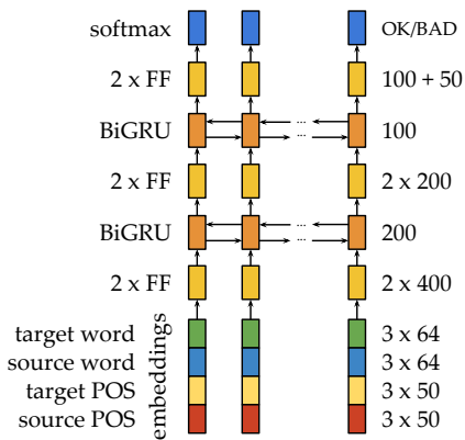
Figure 2: Architecture of our NEURALQE system.
