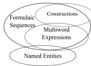
Figure 1: Multiword Terminology
