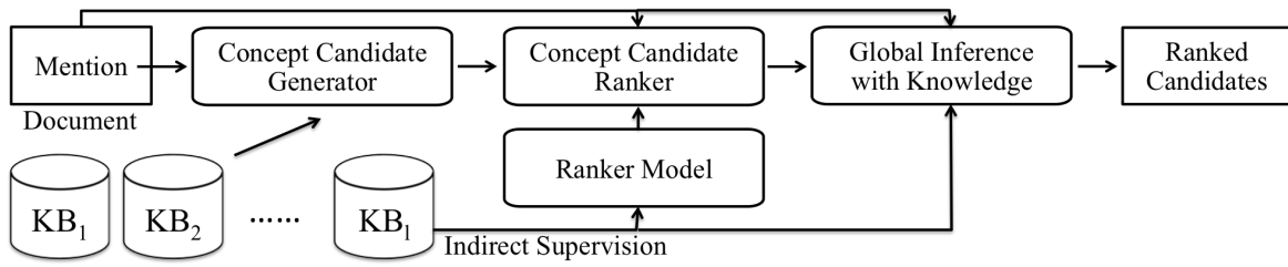
Figure 2: Algorithmic components of our system.
