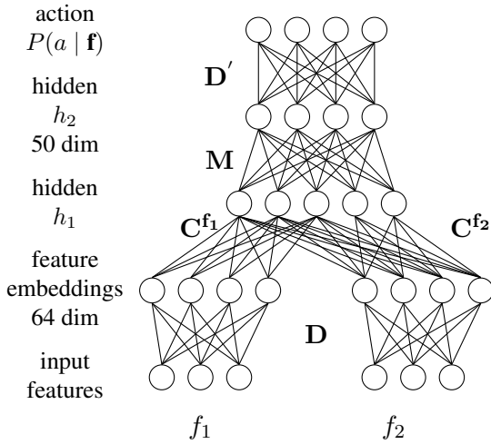
Figure 3: Basic architecture of our NN models
