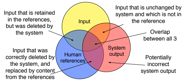
Figure 1: Metrics that evaluate the output of monolingual text-to-text generation systems can compare system output against references and against the input sentence, unlike in MT metrics which do not compare against the (foreign) input sentence. The different regions of this Venn diagram are treated differently with our SARI metric.
