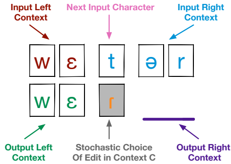
Figure 2: Illustration of a contextual edit process as it pronounces the English word wetter by transducing the underlying /wɛt#ət/ (after erasing #) to the surface [wɛrər]. At the point shown, it is applying the “intervocalic alveolar flapping” rule, replacing /t/ in this context by applying SUBST(r).
