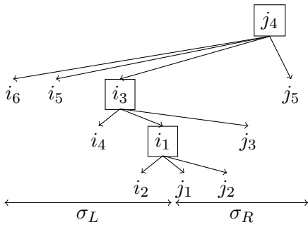
Figure 2: A possible linear tree for string pair (\sigma_L, \sigma_R) , where \sigma_L = i_6i_5i_4i_3i_2i_1 and \sigma_R = j_1j_2j_3j_4j_5 . The spine of the tree consists of nodes j_4, i_3 and i_1 .
