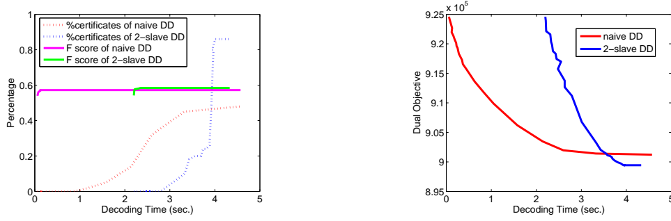
Figure 4: QA sentence dependency tagging using 3-wise CRFs: The F scores, dual objectives, and fraction of optimality certificates relative to decoding time.
