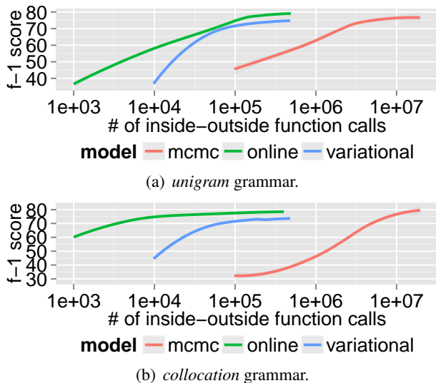
Figure 2: Word segmentation accuracy measured by word token F_1 scores on brent corpus of three approaches against number of inside-outside function call using unigram (upper) and collocation (lower) grammars in Table 1. 6
