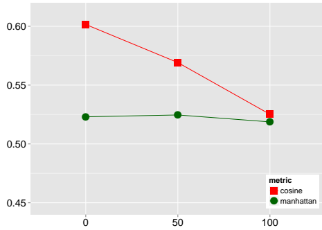
Figure 15: AP, metric / n. of skipped dim.
