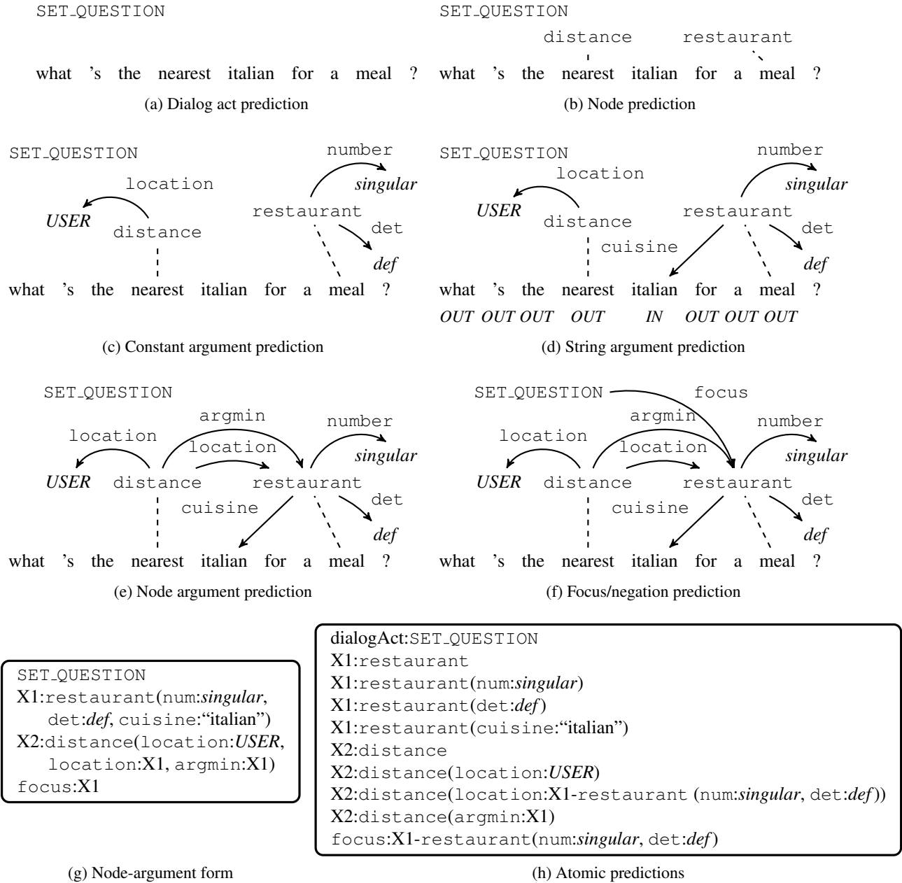
Figure 2: Semantic parsing decomposition.
