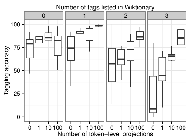
Figure 4: Relative influence of token and type constraints on tagging accuracy in the \hat{y}_{\text{wik.}}^{\text{CRF}}+\text{C}+\text{L} model. Word types are categorized according to a) their number of Wiktionary tags (0,1,2 or 3+ tags, with 0 representing no Wiktionary entry; top-axis) and b) the number of times they are token-constrained in the training set (divided into buckets of 0, 1-9, 10-99 and 100+ occurrences; x-axis). The boxes summarize the accuracy distributions across languages for each word type category as defined by a) and b). The horizontal line in each box marks the median accuracy, the top and bottom mark the first and third quantile, respectively, while the whiskers mark the minimum and maximum values of the accuracy distribution.
