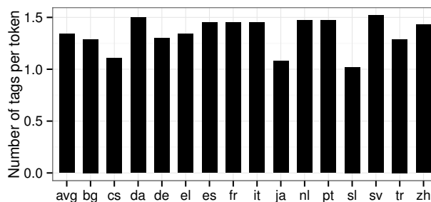
Figure 3: Average number of licensed tags per token on the target side of the bitext, for types in Wiktionary.
