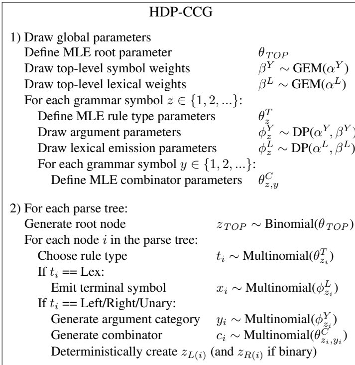
Figure 1: The HDP-CCG has two base distributions, one over the space of categories and the other over words (or tags). For every grammar symbol, an argument distribution and emission distribution is drawn from the corresponding Dirichlet Processes. In addition, there are several MLE distributions tied to a given symbol for generating rule types, combinators and lexical tokens.
