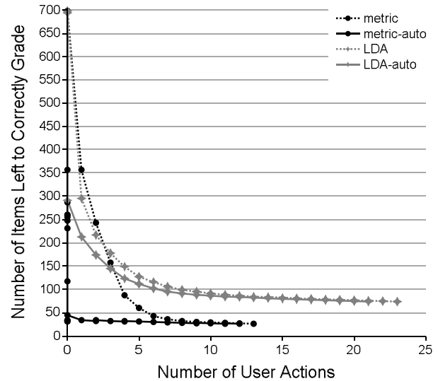
Figure 4. Number of items left to grade or correct out of 698 after each macro user action for G1, question 4.
