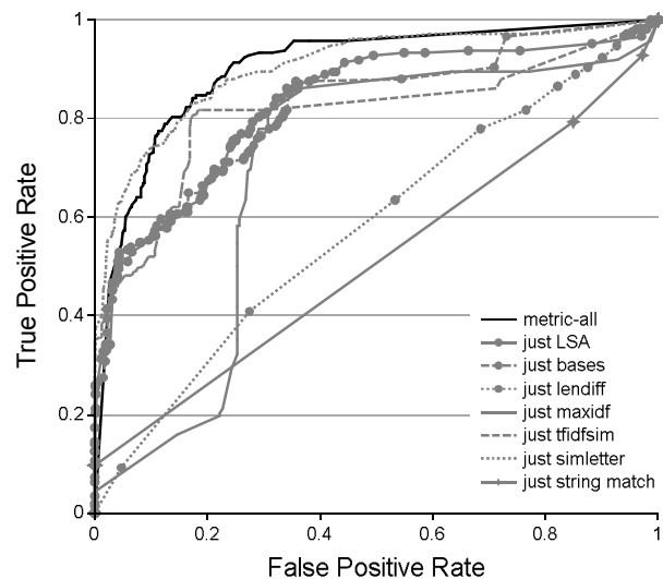
Figure 2. ROC on the grouping task for LR trained on individual features as well as all features.
