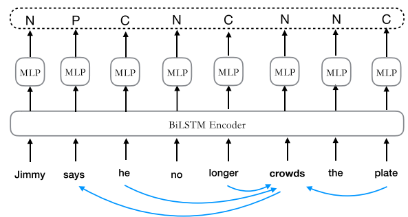
Figure 4: Predicting the link type of each word in a sentence. Blue lines denote dependency arcs between words in the sentence and the predicate crowds .
