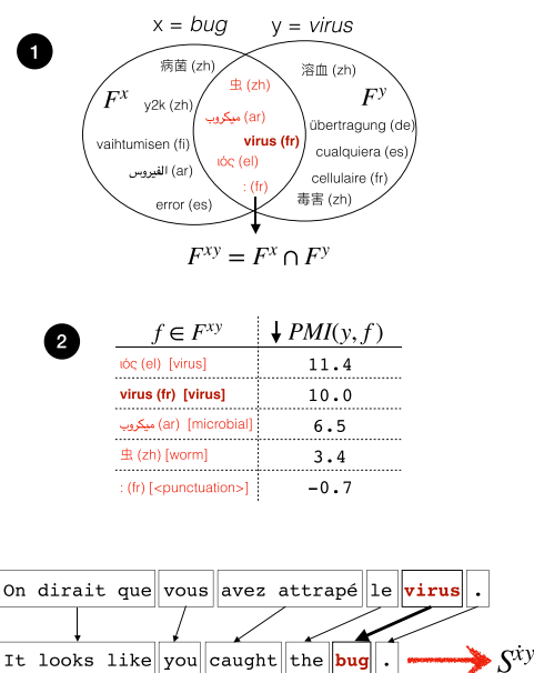
Figure 2: Extracting sentences containing the noun x = \text{bug} in its y = \text{virus} sense for PSTS set S^{\bar{x}y} . In Step 1, the set F^{xy} of translations shared by bug and virus is enumerated. In Step 2, the translations f \in F^{xy} are ranked by PMI(y, f) , in order to prioritize bug 's translations most ‘characteristic’ of its meaning in the virus sense. In Step 3, sentences where bug has been aligned to the French translation f = \text{virus} are extracted from bitext corpora and added to the set S^{\bar{x}y} .
