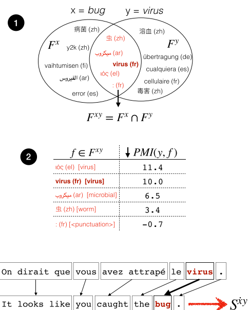
Figure 2: Extracting sentences containing the noun x = \text{bug} in its y = \text{virus} sense for PSTS set S^{\bar{x}y} . In Step 1, the set F^{xy} of translations shared by bug and virus is enumerated. In Step 2, the translations f \in F^{xy} are ranked by PMI(y, f) , in order to prioritize bug ’s translations most ‘characteristic’ of its meaning in the virus sense. In Step 3, sentences where bug has been aligned to the French translation f = \text{virus} are extracted from bitext corpora and added to the set S^{\bar{x}y} .
