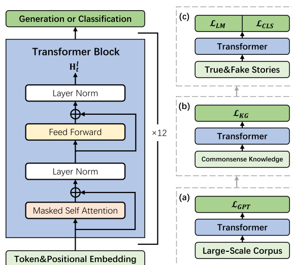
Figure 1: Transformer block architecture (left) and training framework (right). We divide the whole training framework into the following three stages. Train the language model (a) with a large-scale corpus, in which stage we directly inherit the pretrained model parameters from Radford et al. (2019), (b) with commonsense knowledge from external knowledge bases, and (c) with true and auto-constructed fake stories by multi-task learning for story generation and classification. \mathcal{L}_{GPT} , \mathcal{L}_{KG} , \mathcal{L}_{LM} , and \mathcal{L}_{CLS} are the corresponding loss functions in different stages, respectively.
