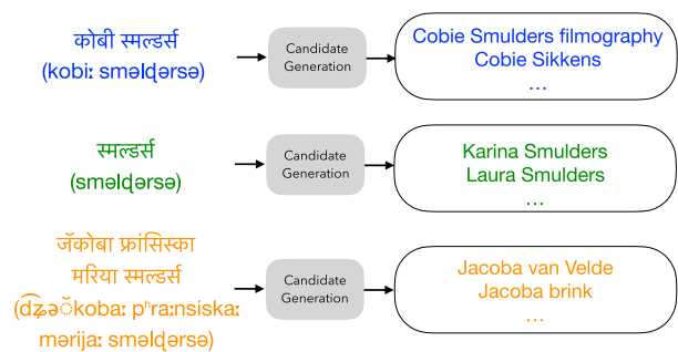
Figure 1: The candidate generation process for various mentions corresponding to the gold entity “Cobie Smulders”. Strings on the left are mentions in the document, and the pronunciation in IPA of each string is written below it. The candidate entities in the English KB generated by the candidate generation model are shown on the right.
