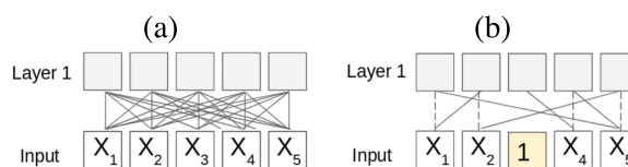
Figure 2: Finding a good input restriction: (a) Every attention head in the first layer could potentially attend to any input bit. (b) Perhaps surprisingly, one can fix a small number of input bits in such a way that each layer-1 attention head can only possibly attend to c (here, c = 1 ) inputs, and ignores all other inputs. Each activation vector y_j^{(1)} in the first layer then only depends on the H \cdot c inputs that its H (here, H = 1 ) attention heads can attend to, plus the input x_j that feeds into it via a skip-connection.
