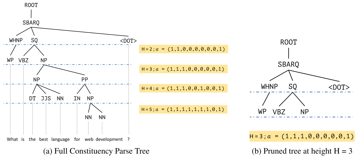
Figure 2: The constituency parse tree serves as an input to the syntactic encoder (Section 3.3). The first step is to remove the leaf nodes which contain meaning representative tokens (Here: What is the best language . . . ). H denotes the height to which the tree can be pruned and is an input to the model. Figure 2(a) shows the full constituency parse tree annotated with vector \mathbf{a} for different heights. Figure 2(b) shows the same tree pruned at height H = 3 with its corresponding \mathbf{a} vector. The vector \mathbf{a} serves as a signalling vector (Section 3.4.2) which helps in deciding the syntactic signal to be passed on to the decoder. Please refer Section 3 for details.
