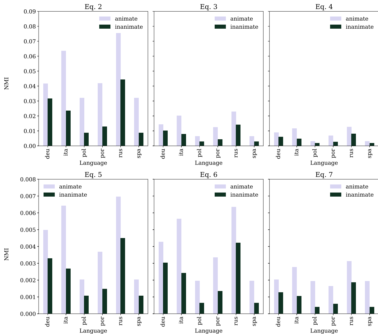
Figure 5: The normalized mutual information (NMI) between the grammatical genders of a) inanimate and b) animate nouns and the verbs that take those nouns as direct objects. Each subplot contains NMI(G_i^\ell, D_i^\ell) and NMI(G_a^\ell, D_a^\ell) , calculated using a single normalizer, for each language \ell \in \{de, it, pl, pt, ru, es\} .
