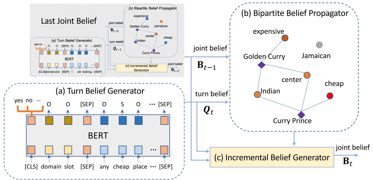
Figure 2: The architecture of the proposed ReDST model, which comprises (a) a turn belief generator, (b) a bipartite belief propagator, and (c) an incremental belief generator. The turn belief generator will predict values for domain slot pairs. Together with the last joint belief, the beliefs will be aggregated via the bipartite belief propagator based on the database structure. Then the incremental belief generator infers the final joint belief.
