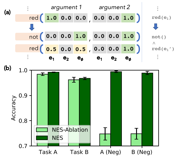
Figure 9: Negation with NES. (a) We visualize one way in which NES can handle coordination for non-intersective modifiers (e.g., attribute negation) by leveraging the background event e_\theta . NES soft routing leads to a modified event argument input e'_1 attending over e_1 and e_\theta , enabling the red classifier to output the opposite prediction (now, output score = 1.0 if original e_1 is not red). (b) NES performance on Task A and B negation variants remains consistent. Ablation (Section 4.1.4) highlights the impact of the event routing mechanism.
