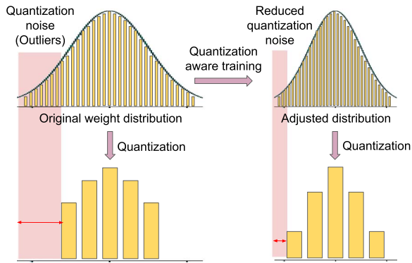
Figure 4: Quantization.
