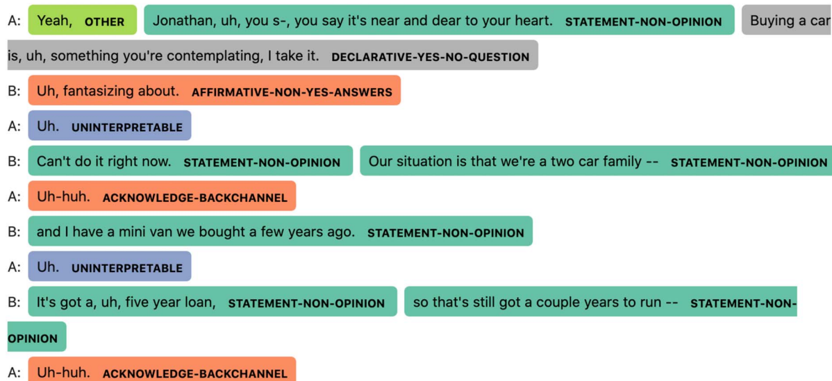
Figure 1: An illustration of dialog acts in a Switchboard conversation. Note how the speaker turns may consist of multiple dialog acts, indicating a different function for each utterance. Dialog act annotation allows us to segment the conversation into meaningful units that can be used for downstream processing in spoken language understanding (SLU) applications.
