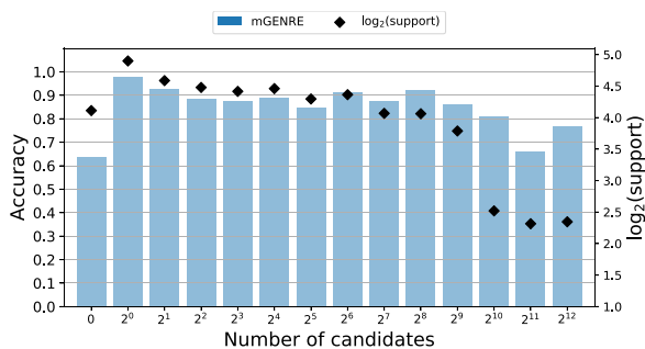
Figure 3: Results of mGENRE on Mewsl-9 by the number of retrieved candidates.
