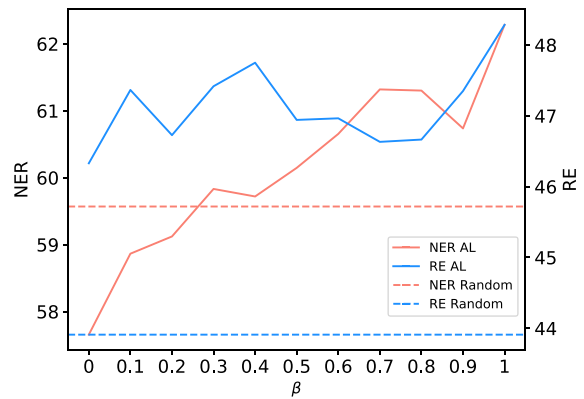
(a) ScieRC
