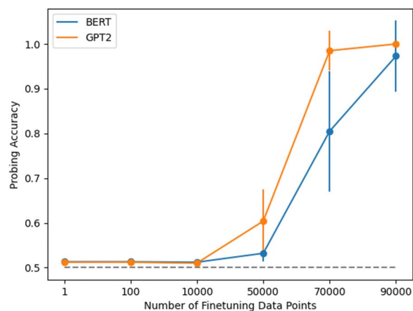
Figure 2: Probing accuracy after finetuning a pre-trained LM on our (coordinated) referential opacity dataset with different numbers of finetuning examples. The mean and the standard deviation across 10 seeds are plotted. For clarity in visualizing the trend, the x-axis is not in linear scale.
