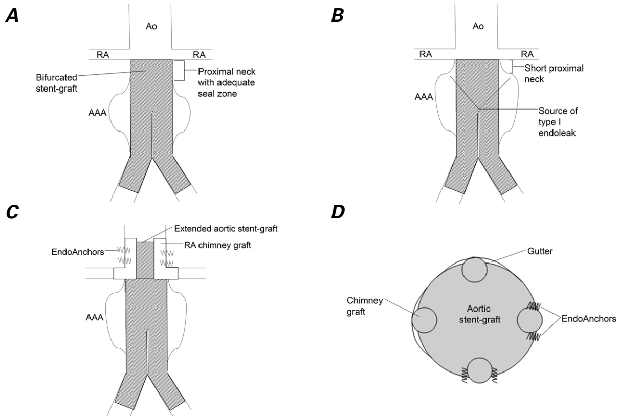
Fig. 1 Schematic drawings show coronal views of A ) an ideal infrarenal neck length and adequate seal zone, compared with B ) a short proximal neck and an inadequate seal zone, which creates a high risk for type I endoleak. C ) An extended aortic stent-graft, chimney grafts, and EndoAnchors securely seal the aneurysm. D ) The transverse view shows EndoAnchors at the 3 and 6 o'clock positions alongside the chimney graft. Gutters at 9 and 12 o'clock may allow persistent flow into the aneurysmal sac.
