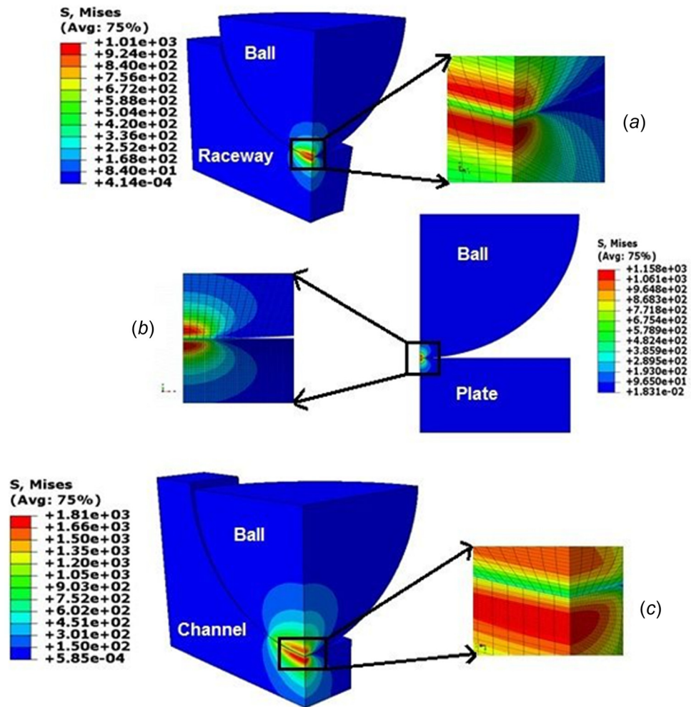
Fig. 1 von Mises stress contours for (a) 3D ball–raceway contact inside radially loaded 6309 DGBB, (b) axisymmetric ball–plate contact, and (c) 3D ball–inside–channel model
