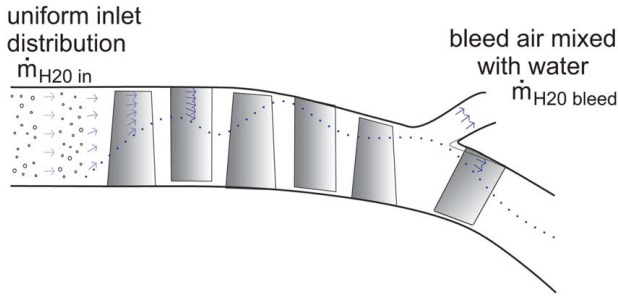
Fig. 1 Schematic of water distribution through the core compressor of an aero engine and its removal via the casing bleed slot
