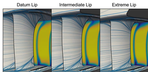
Fig. 13 CFD results for operation at the design point showing suction surface streamlines and stagnation pressure loss contours for datum, intermediate, and extreme lip designs
