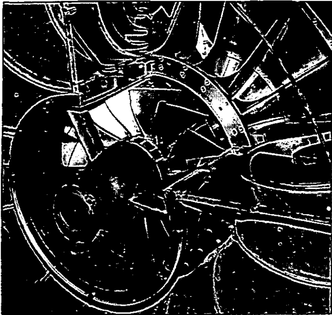
Figure 6. Inlet section of the HeS 3B showing inducer and centrifugal compressor
