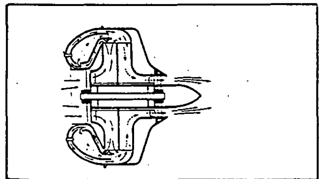
Figure 4. Patent drawing of Hahn showing combustor located in front of centrifugal compressor.
