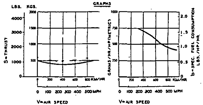
Figure 9. Performance characteristics of the He S3B.
