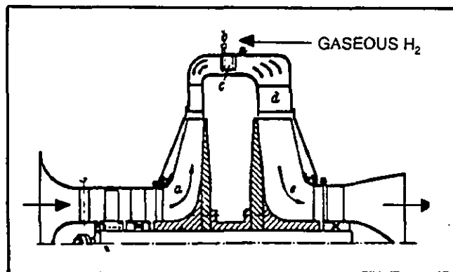
Figure 3. HeS 1 Demonstrator run on hydrogen fuel
