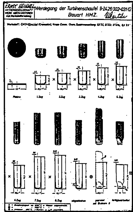
Figure 20. Ingenious method of developing air cooled turbine blade starting with a circular plate 25 mm dia.
