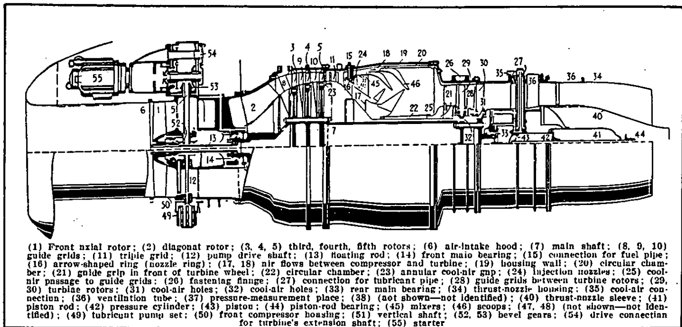
Figure 14. Layout of the advanced HeS 011 engine (Neville and Silsbee, 1948).
