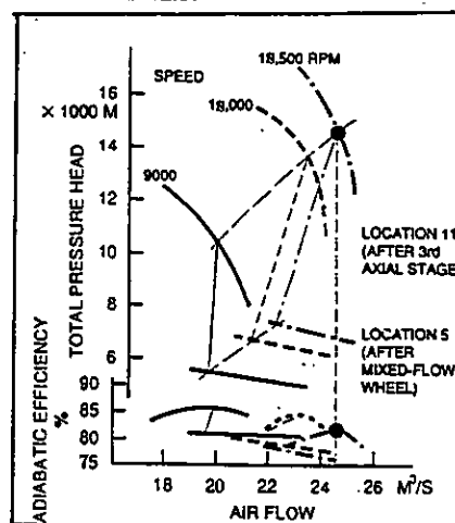
Figure 16. HeS 011 Compressor Map (Bentele, 1991)
