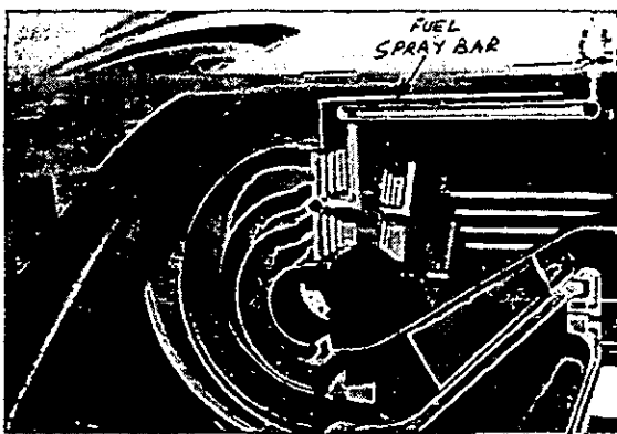
Figure 7. Combustor section of the HeS 3B.
