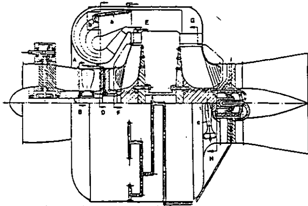
Figure 5. Layout of the HeS 3B flight engine (Gunston 1995).
