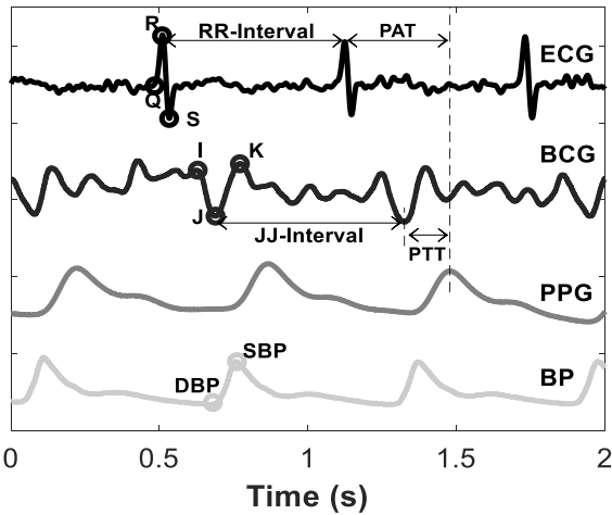
Figure 1. An example of simultaneous recording of ECG, BCG, PPG, and BP signals. IJK complex of BCG signal and QRS complex of ECG signal denoted.
