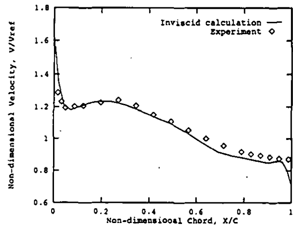
Fig. 4, Suction surface velocity comparison \beta_1 = 40^\circ
